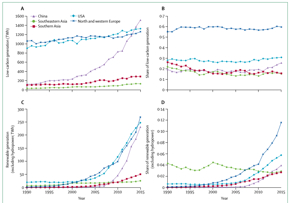
Figure 16: Renewable and zero-carbon emission electricity generation
