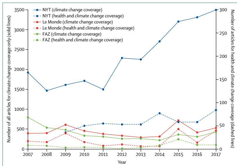
Figure 26: Newspaper reporting of climate change and health and climate change in the NYT, Le Monde, and FAZ in 2007–17
